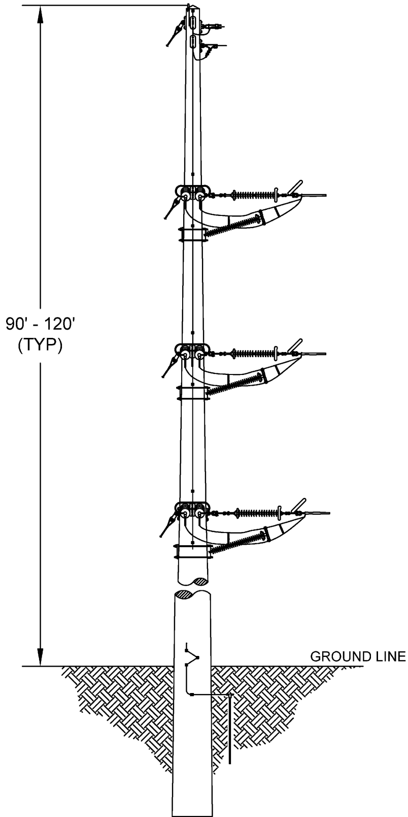
Figure 1-3 Typical Monopole Deadend Structure Reata Station to Roadrunner Crossing Wind 345 kV Transmission Line Lone Star Transmission
